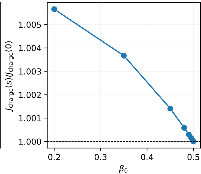
Complete PH charge resolvent
