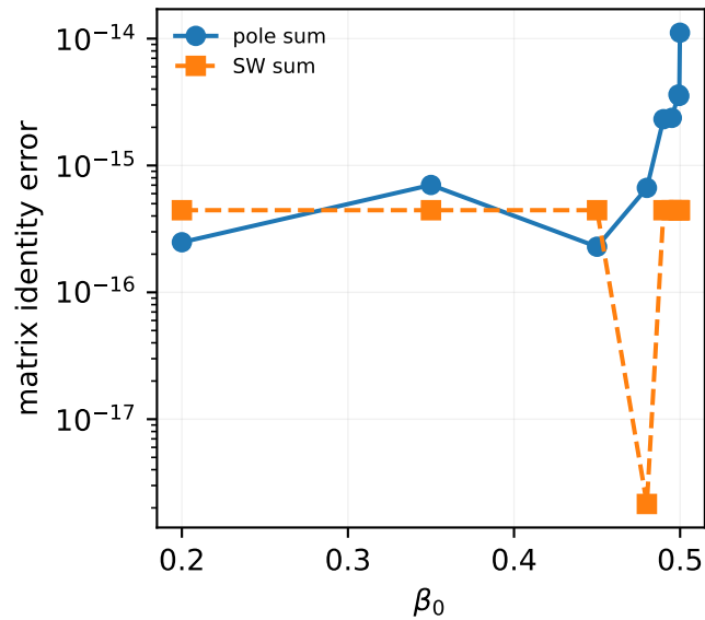
Singular pieces cancel
