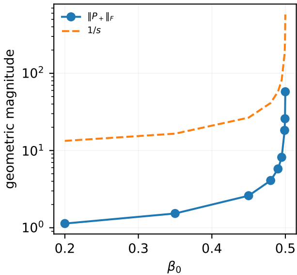
Individual projector growth
