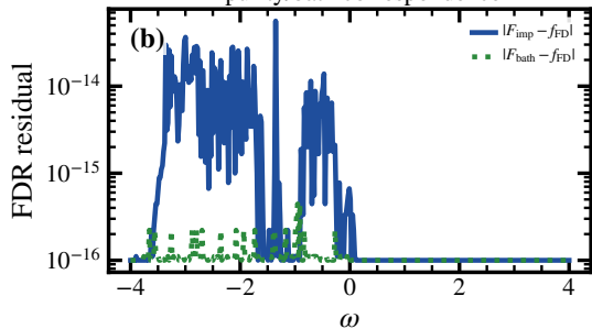
Physical spectrum ( \beta_0 = 0.45 , \delta_{\text{br}} = 0.015 , causal)
