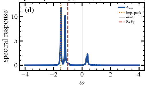
Physical spectrum ( \beta_0 = 0.45 , \delta_{\text{br}} = 0.015 , causal)
