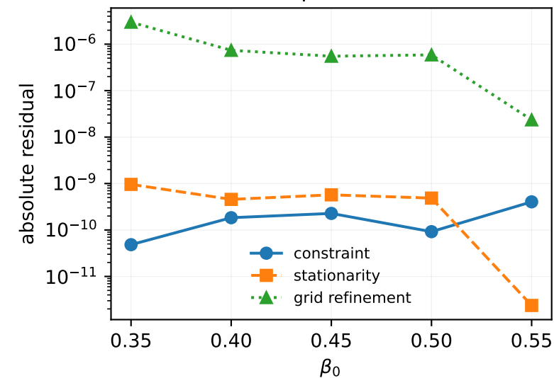
Saddle and quadrature checks
