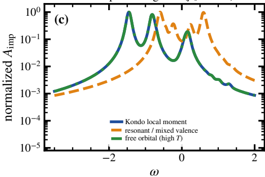
Three spectral regimes ( \beta_0 = 0.25 )
