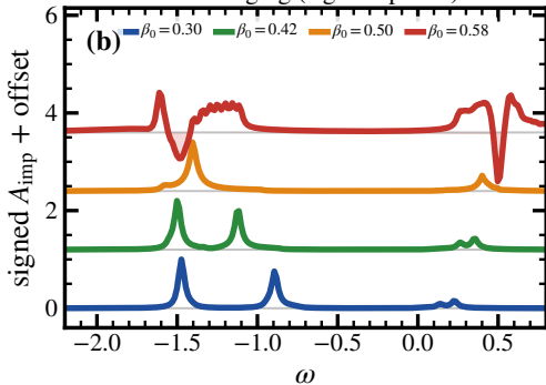
Peak merging (signed spectra)
