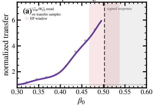
SBMF spectral-weight transfer
