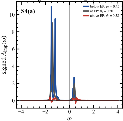
No negative DOS below \beta_{\text{EP}} ( \eta = 0.015 )
