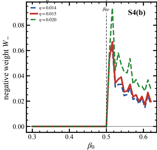
Sign defect turns on only after the EP
