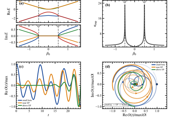
FIG. 1. Full 4 \times 4 non-Hermitian impurity kernel: spectrum, condition number, and real-time dynamics. All panels use the gauge-fixed frozen-kernel convention \tilde{\beta} = |\beta_0|r with \epsilon_\xi = -U/2 = -1.0 , U = 2.0 , and T_b = 0.1 . The plotted eigenvalues and eigenvectors are computed from the full rotated 4 \times 4 kernel of Eq. (40), not from the isolated impurity block. (a) Real and imaginary parts of the four eigenvalues of \tilde{H}(k=0) versus \beta_0 . The representative finite-drive local EPs occur at |\beta_0| \simeq 0.50 ; double-root tracking gives \beta_{0,\text{proj}}^{\text{EP}} = 0.4975 , while the discrete grid peaks at the adjacent point \beta_0 = 0.5025 ( \Delta\beta_0 = 0.0075 ). (b) Condition number \kappa_{\text{imp}} = \|R\| \|R^{-1}\| , using the same eigenvector normalization throughout the scan. The finite- |\beta_0| peaks locate eigenvector coalescence; the origin is a normal degeneracy and is not interpreted as an EP. (c) Survival-amplitude dynamics for representative points below, at, and above the EP, plotted on a common solver time window. (d) Corresponding phase portraits. The change from oscillatory motion to critical coalescence and then to broken-regime overdamped response is the time-domain signature of the 4 \times 4 finite-drive EP.
