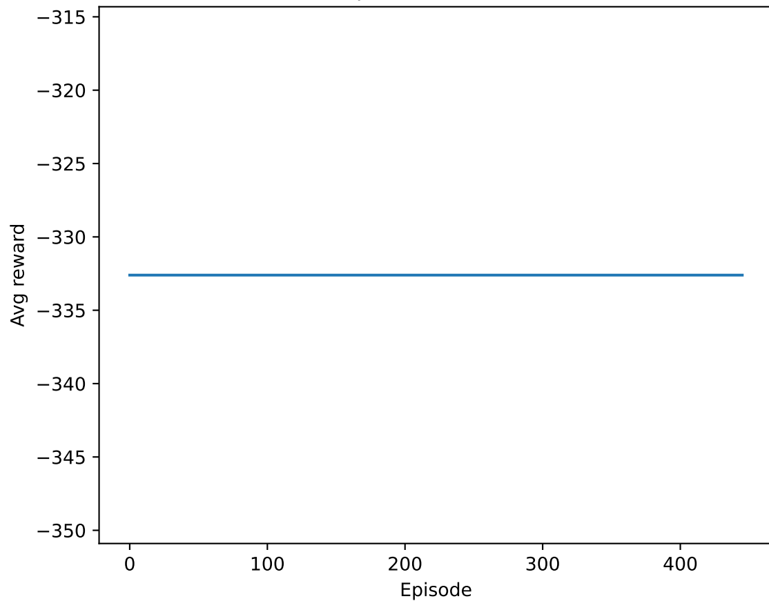
Episode Rewards
