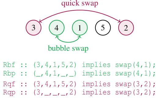
Figure 1: Examples of full (f) and partial (p) advice from C_{\text{bubble}} (b) and C_{\text{quick}} (q) on (3, 4, 1, 5, 2) .
