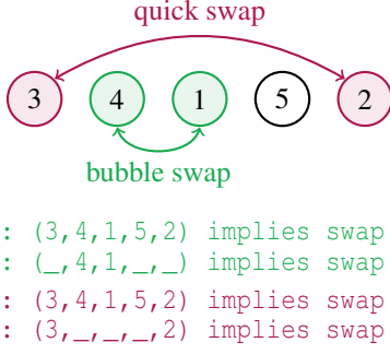
Figure 1: Examples of full (f) and partial (p) advice from C_{\text{bubble}} (b) and C_{\text{quick}} (q) on (3, 4, 1, 5, 2) .
