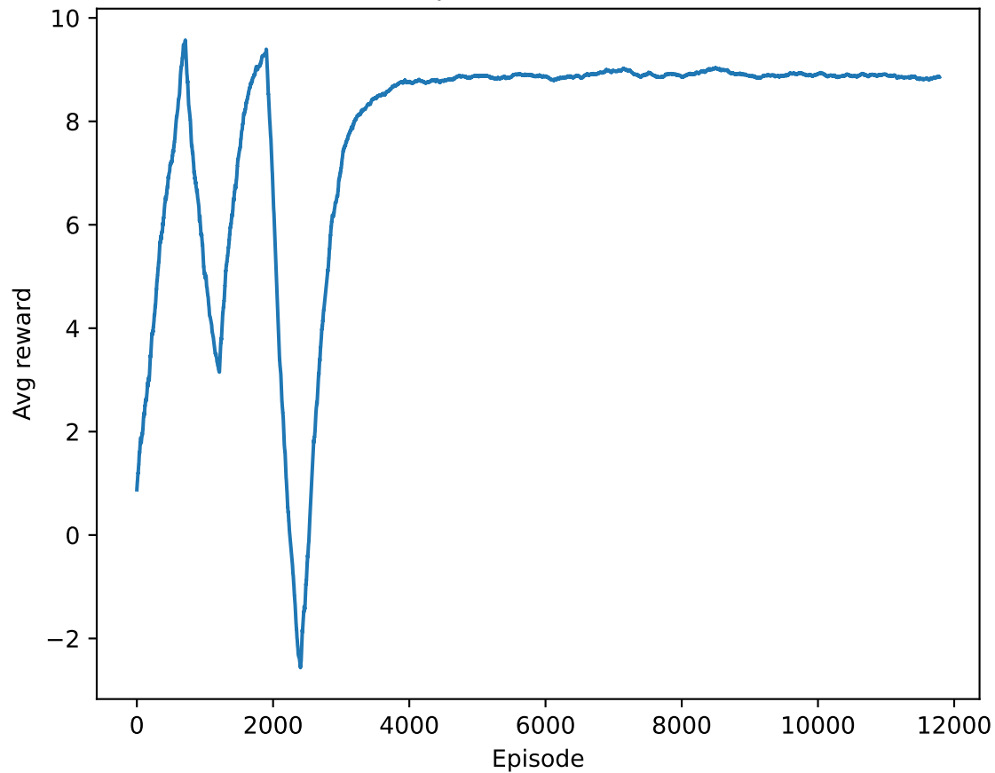
Episode Rewards
