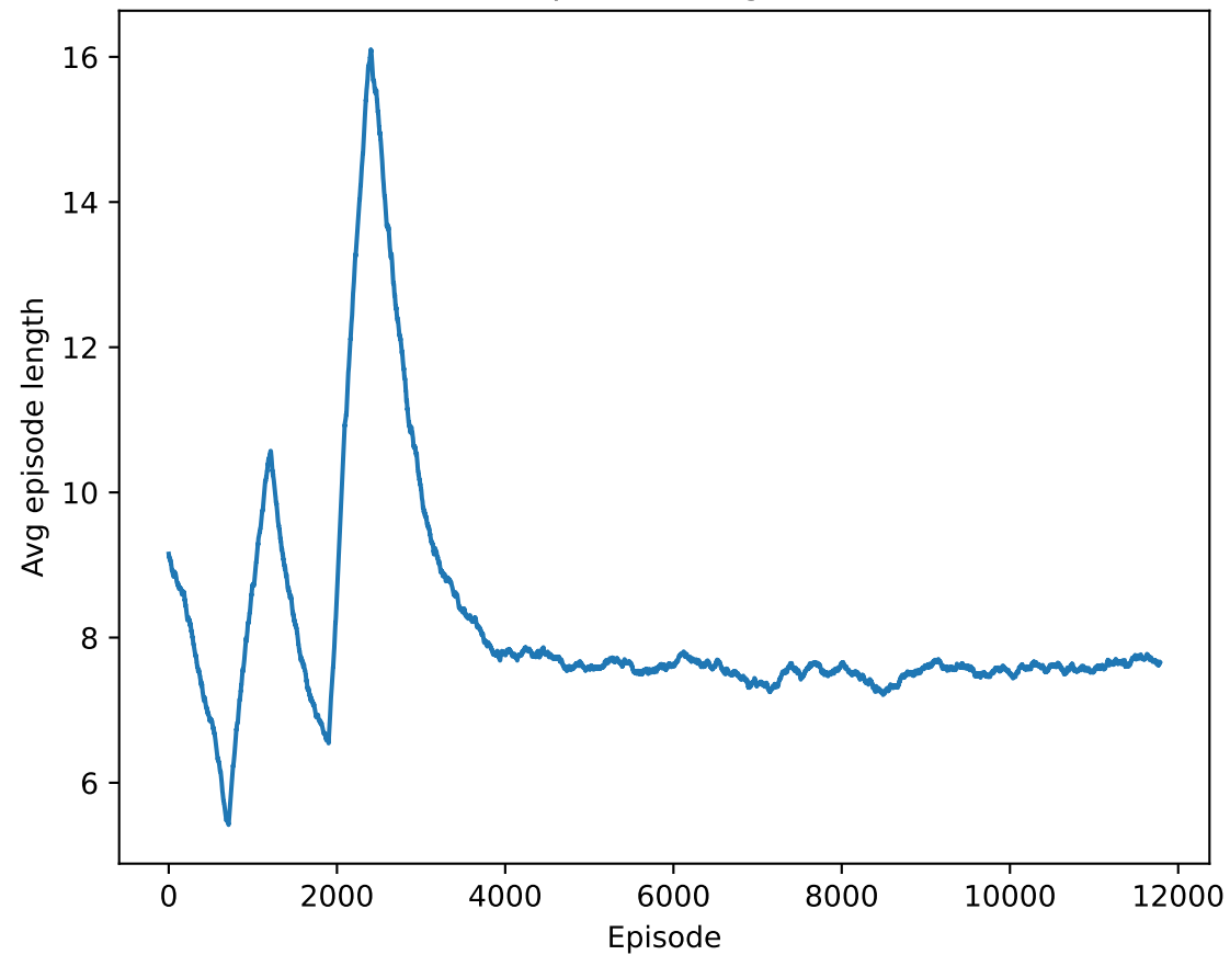
Episode Length
