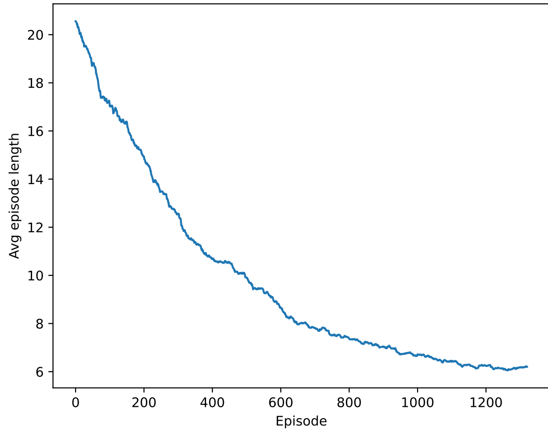
Episode Length
