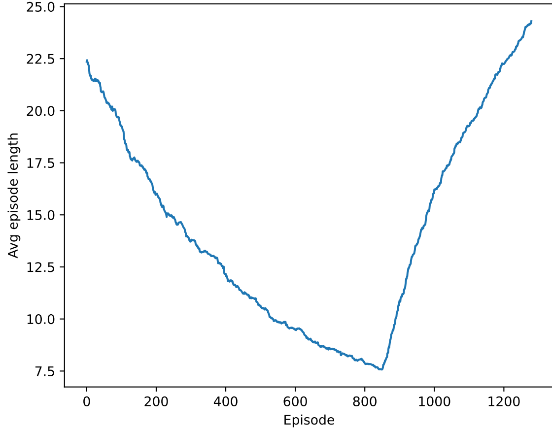
Episode Length
