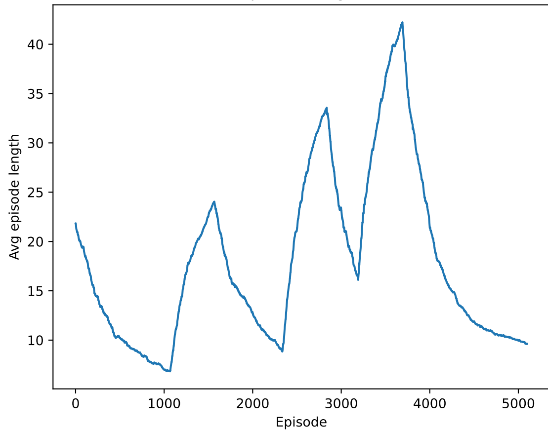
Episode Length
