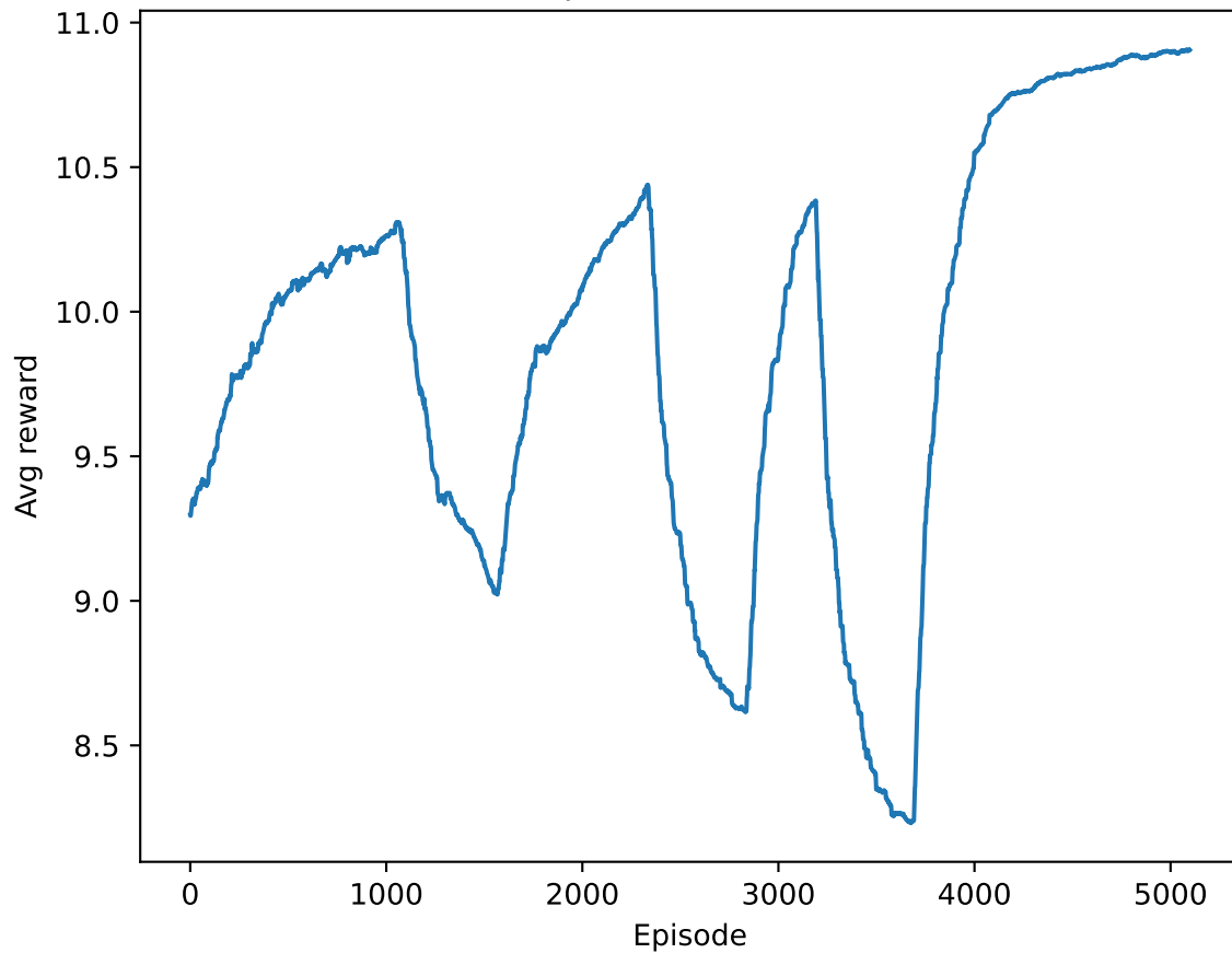
Episode Rewards
