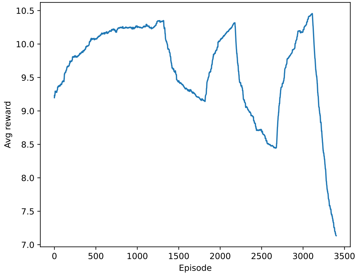
Episode Rewards
