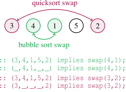
Figure 1: Examples of full (f) and partial (p) advice from P_{\text{bubble}} (b) and P_{\text{quick}} (q) on state (3, 4, 1, 5, 2) .
