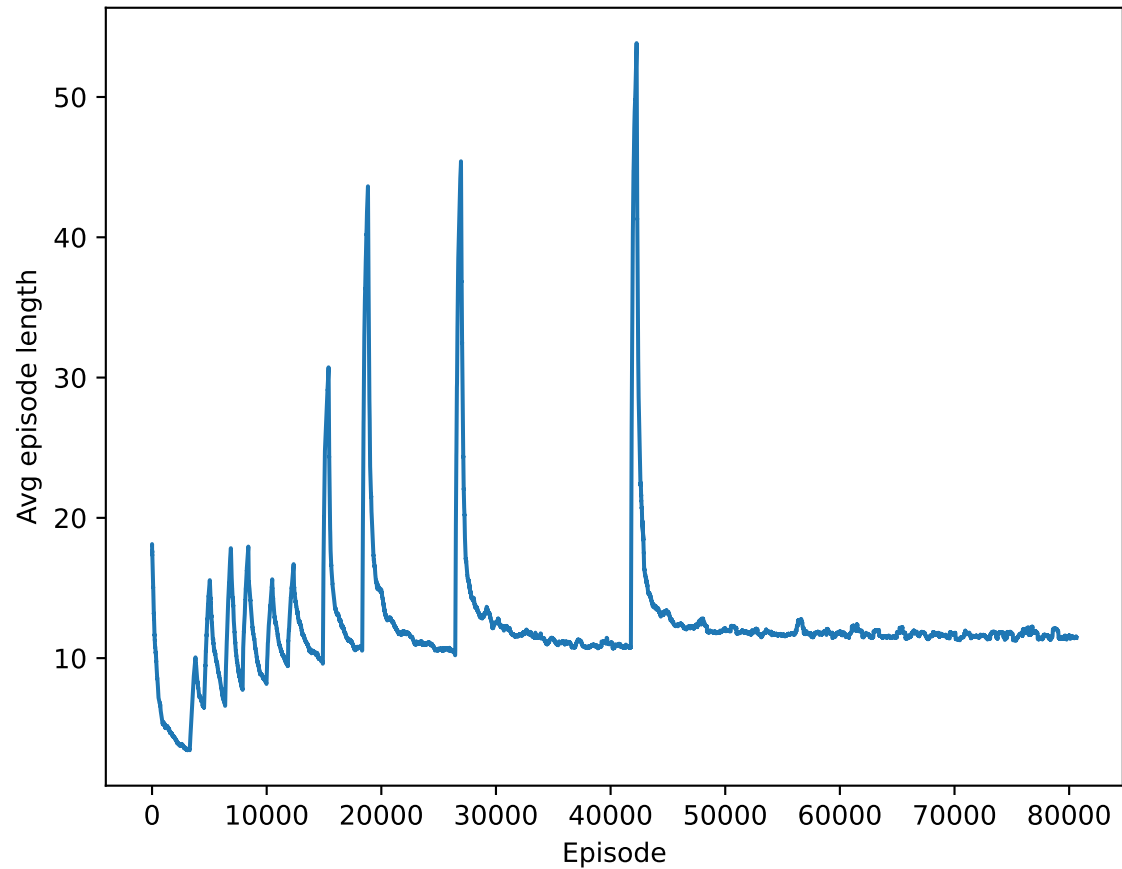
Episode Length
