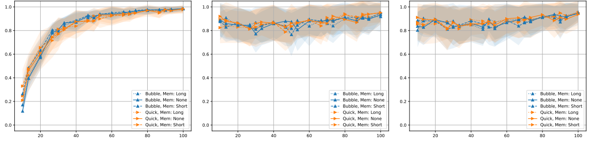
Figure 5: Coaching fidelity against advice coverage for reactive (left), proactive (middle) and reflexive (right) coaching.
