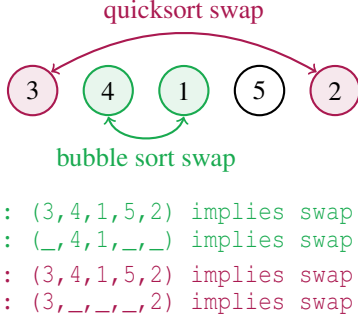
Figure 1: Examples of full (f) and partial (p) advice from P_{\text{bubble}} (b) and P_{\text{quick}} (q) on state (3, 4, 1, 5, 2).
