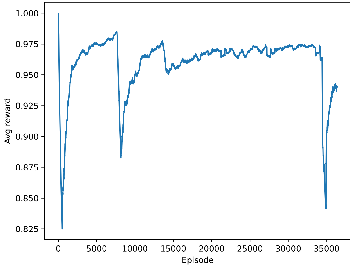
Episode Rewards
