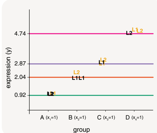
Figure 12. Expected gene expression is modelled by a group factor and two additional factors that are not of interest (lane and technician). The design matrix excludes the intercept term for the first factor added to the function. Only lines reflecting the first 4 parameters are drawn in the plot, representing the mean gene expression of groups A, B, C and D in lane L1 and with handling technician I. Samples are labelled by their sequencing lane (L1 or L2), and coloured black if they are processed by technician I, yellow if they are processed by technician II.
