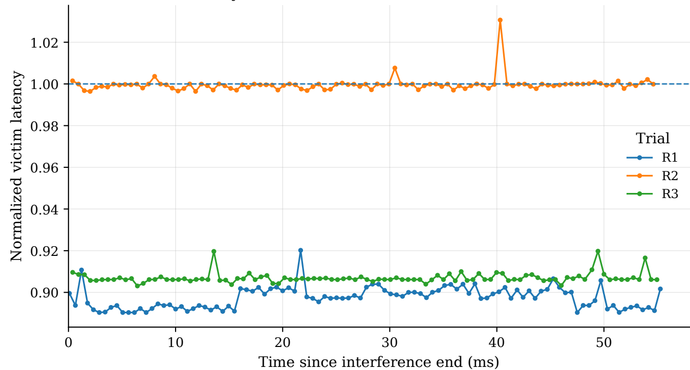
Tesla T4: L2 recovery across three 100 ms trials
