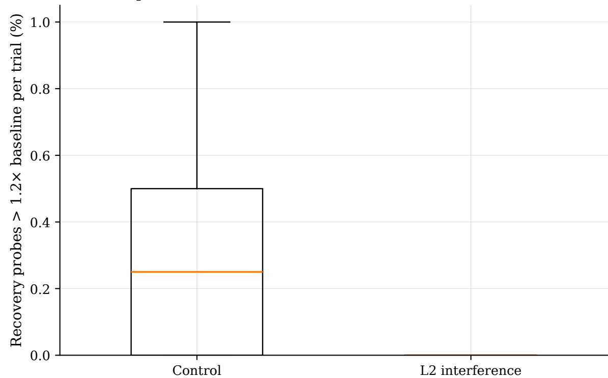
Tesla T4: post-interference tail excursions
