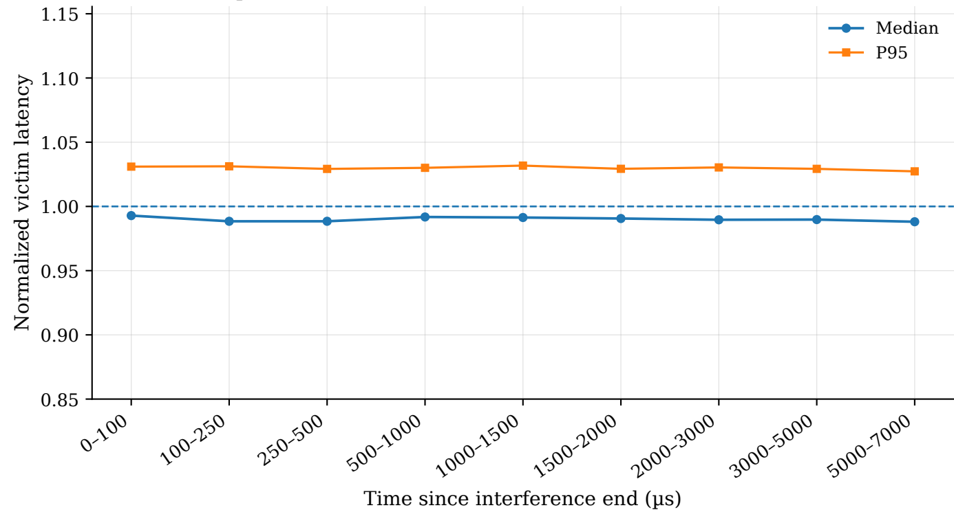
Tesla T4: temporal behavior after L2 interference
