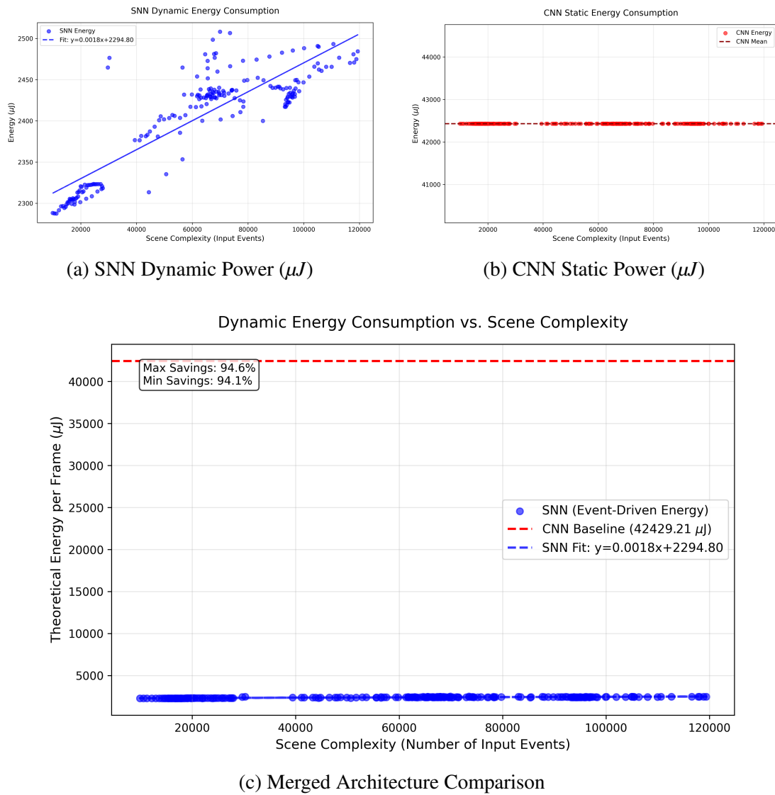
Figure 2.6: Comparison of dynamic power consumption ( \mu J ) between the SNN and CNN architectures relative to the raw event count of the input scene. The isolated SNN graph (a) demonstrates strong linear scaling ( R^2 = 0.7514 ), validating its event-driven efficiency, whereas the CNN (b) consumes a massive static overhead.
