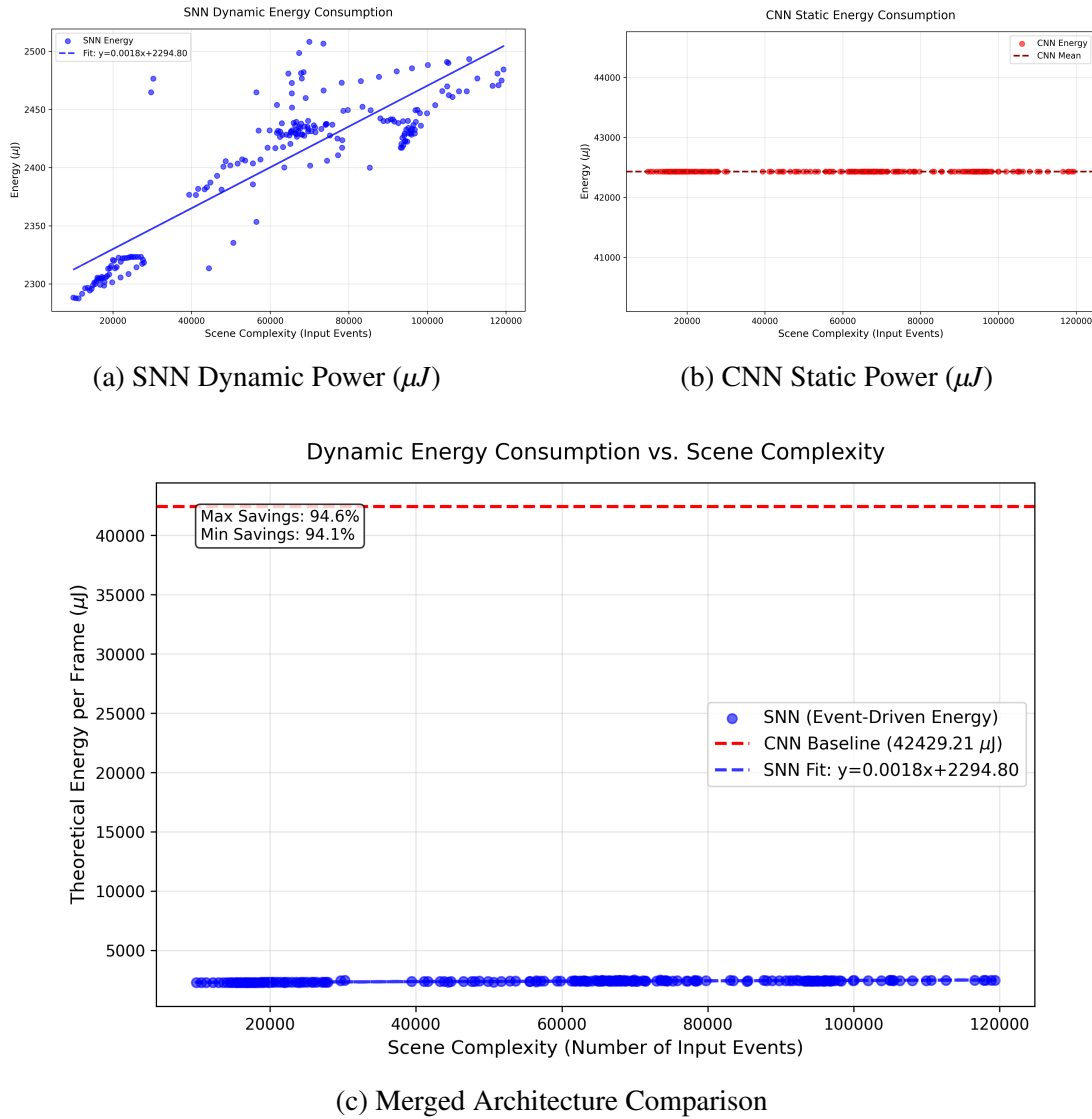
Figure 3.6: Comparison of dynamic power consumption ( \mu J ) between the SNN and CNN architectures relative to the raw event count of the input scene. The isolated SNN graph (a) demonstrates strong linear scaling ( R^2 = 0.7514 ), validating its event-driven efficiency, whereas the CNN (b) consumes a massive static overhead.
