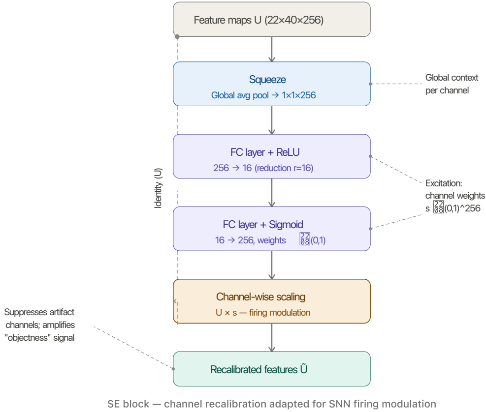
Figure 3.4: The Squeeze-and-Excitation (SE) block [hu2019'se'block] as applied in Stage 3 of the DetectorNX-G3-SNN backbone ( 22 \times 40 \times 256 ).
