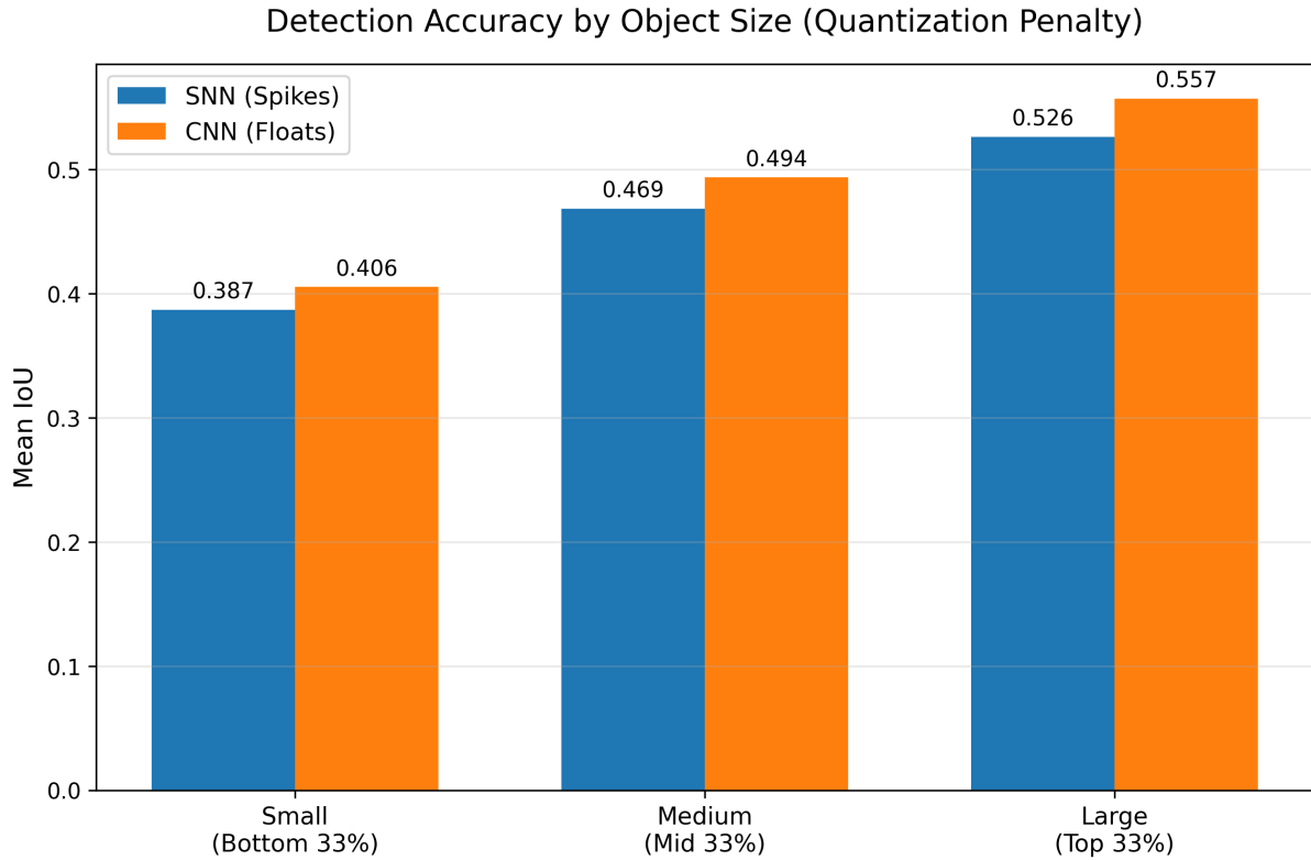
Figure 4.3: Quantisation Error Analysis (Accuracy vs. Object Size) of SNN (Blue) and CNN (Orange). The results invalidate the expected scale-dependent penalty, showing instead that the T = 10 temporal resolution imposes a global geometric drag across all object sizes.
