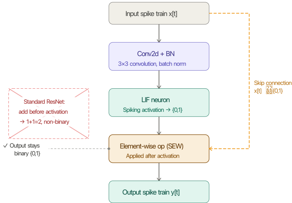
SEWResBlock — element-wise op occurs after spiking activation
