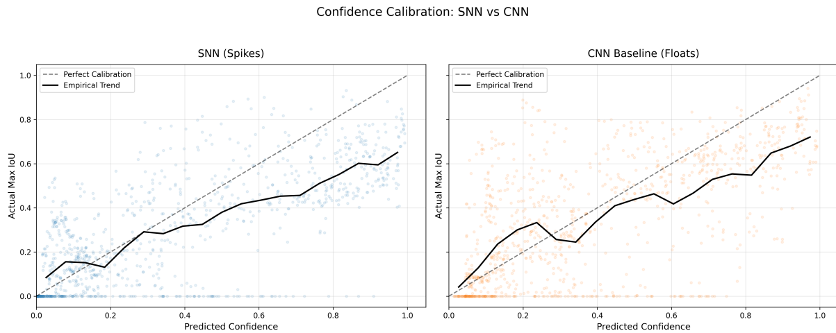
Figure 4.4: Reliability diagrams for the SNN (left) and CNN (right). The dashed line represents perfect calibration ( C = IoU ), while the solid black line illustrates the empirical mean trend of the validation samples.
