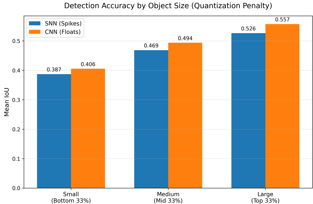
Figure 3.8: Quantization Error Analysis (Accuracy vs. Object Size) of SNN (Blue) and CNN (Orange).
