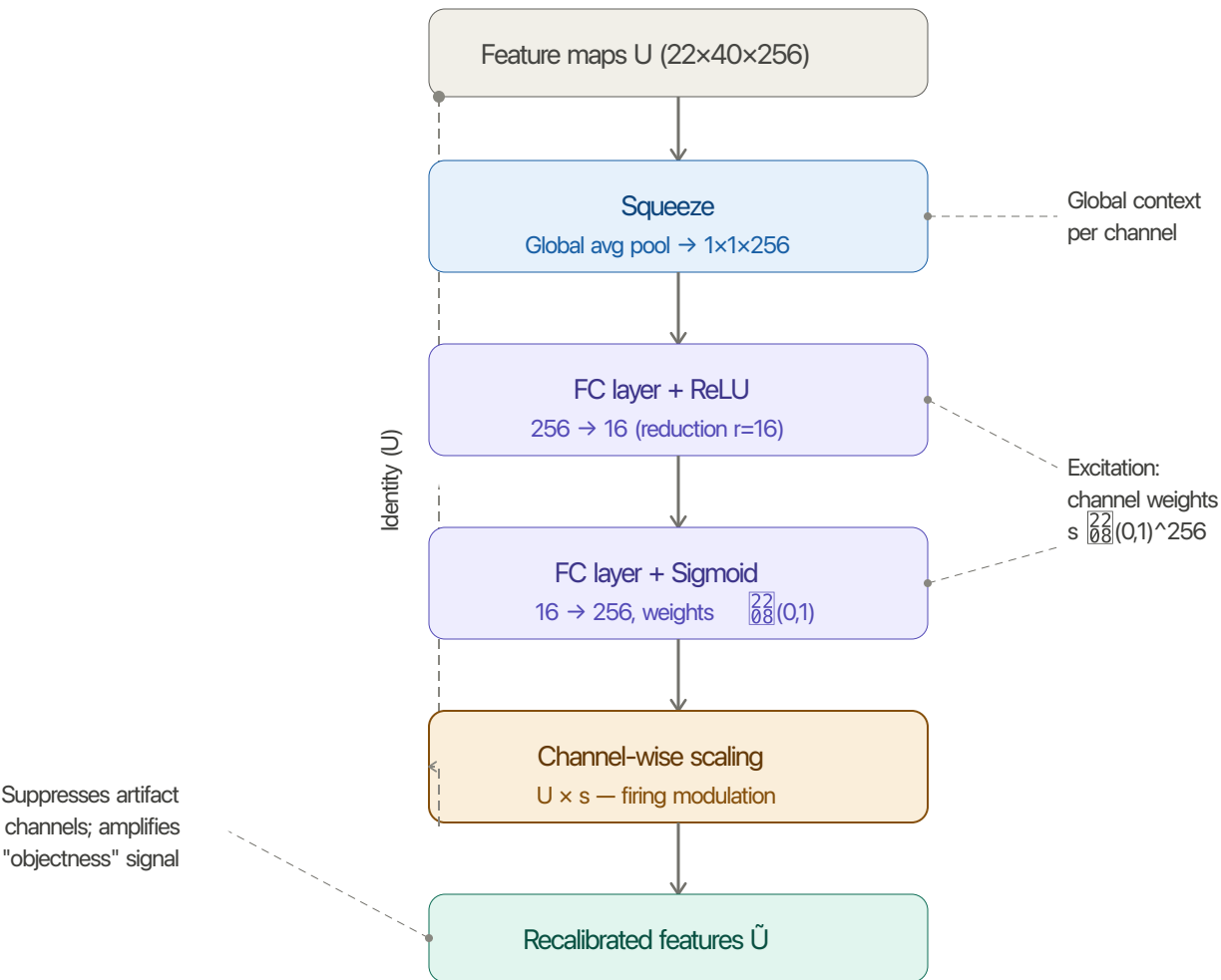
SE block — channel recalibration adapted for SNN firing modulation
