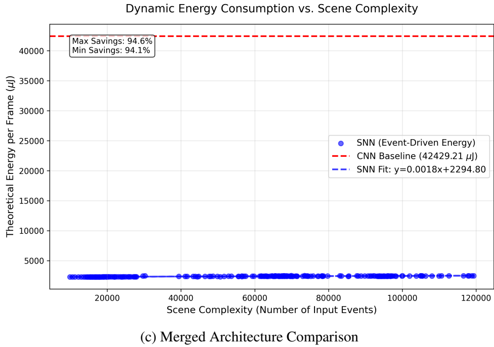
Figure 3.6: Comparison of dynamic power consumption ( \mu J ) between the SNN and CNN architectures relative to the raw event count of the input scene. The isolated SNN graph (a) demonstrates strong linear scaling ( R^2 = 0.7514 ), validating its event-driven efficiency, whereas the CNN (b) consumes a massive static overhead.
