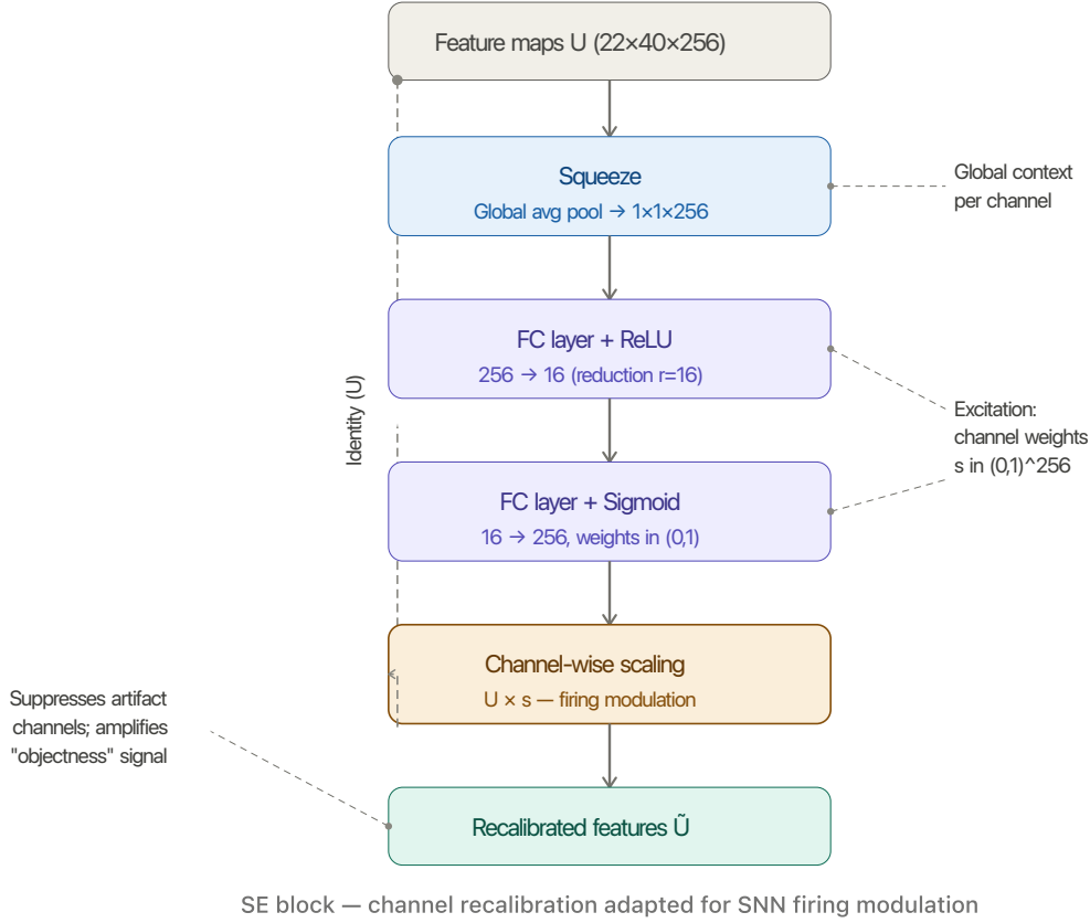
Figure 3.4: The Squeeze-and-Excitation (SE) block [21] as applied in Stage 3 of the DetectorNX-G3-SNN backbone ( 22 \times 40 \times 256 ).
