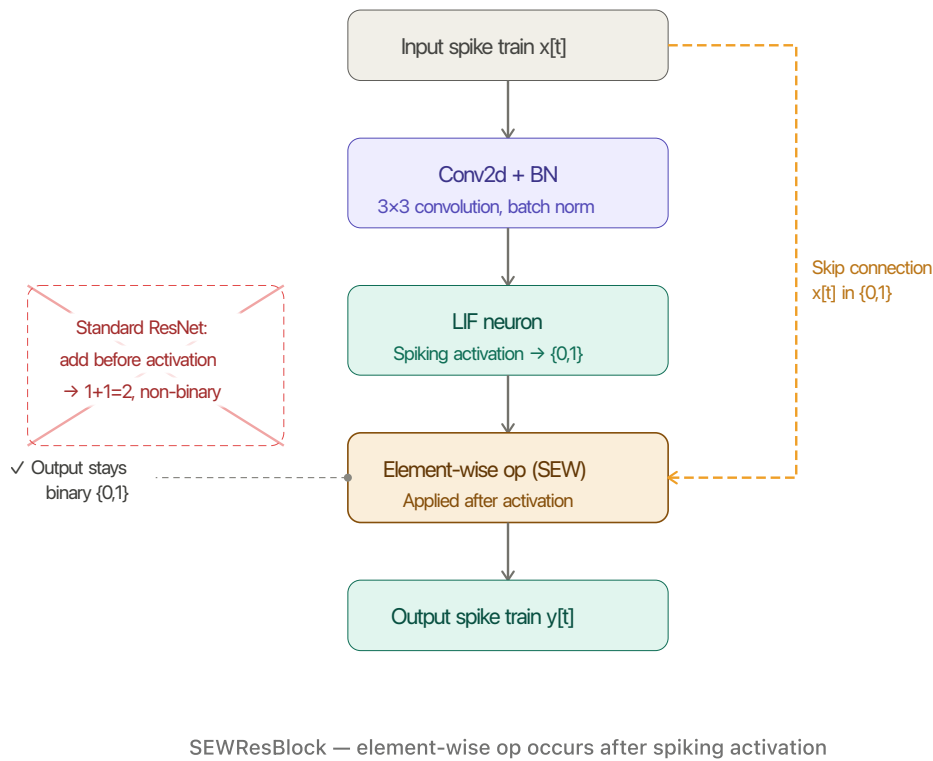
Figure 3.3: The SEW residual block (SEWResBlock) as proposed by Fang et al. [13].
