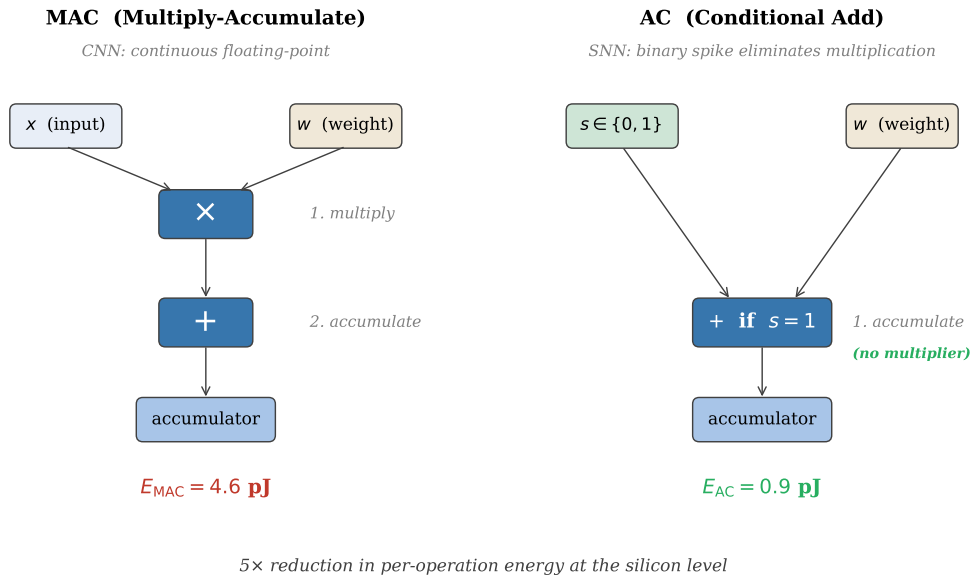
Figure 2.7: The MAC versus AC silicon-level energy distinction. Left : a standard CNN synaptic operation requires a full multiply-accumulate (MAC): the floating-point input x is multiplied by the weight w , then accumulated, costing E_{\text{MAC}} = 4.6 \text{ pJ} per 32-bit operation [20]. Right : a spiking synaptic operation reduces to a single conditional accumulation (AC): the binary spike s \in \{0, 1\} gates whether the weight is added to the running accumulator, eliminating the multiplier entirely. The remaining operation costs E_{\text{AC}} = 0.9 \text{ pJ} — a 5\times reduction in per-operation energy at the silicon level.
