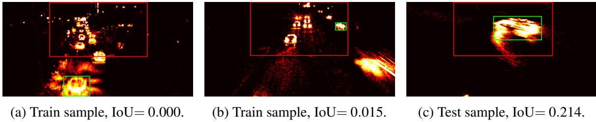
Figure 3.7: Qualitative evidence of Constant Target Bias in G0. Across three raw full-frame samples drawn from the training and test splits, the SNN regression head (red) emits a near-identical large central bounding box while the ground-truth vehicle (green) varies in position and scale between scenes. The marginally higher overlap in (c) arises only because the target vehicle incidentally sits near the image centre where the predicted box anchors, confirming the model has learnt a constant coordinate shortcut rather than extracting vehicle features from the event stream.
