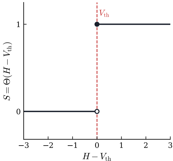
Forward pass
