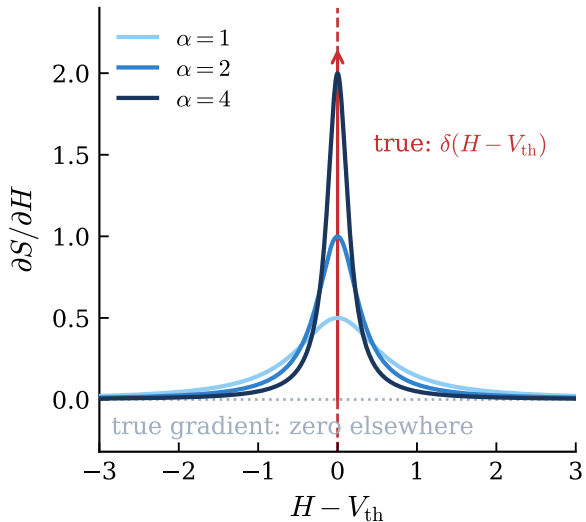
Backward pass
