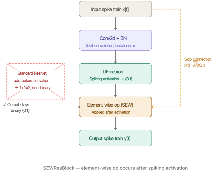
Figure 1.3: The SEW residual block (SEWResBlock) as proposed by [9].
