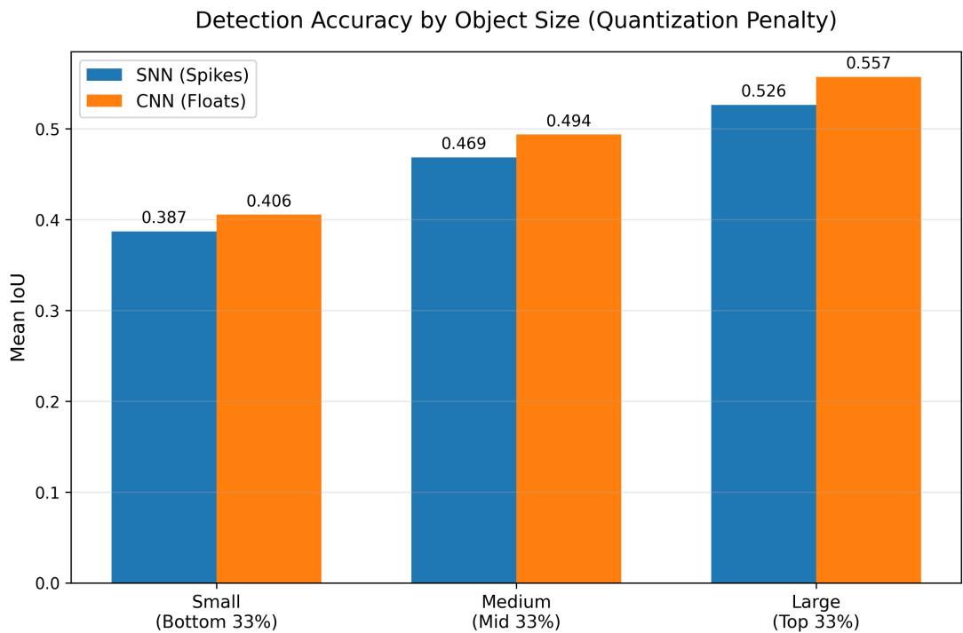
Figure 1.7: Quantization Error Analysis (Accuracy vs. Object Size) of SNN (Blue) and CNN (Orange).
