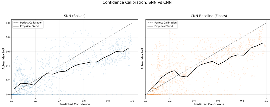
Figure 3.9: Reliability diagrams for the SNN (left) and CNN (right). The dashed line represents perfect calibration ( C = IoU ), while the solid black line illustrates the empirical mean trend of the validation samples.
