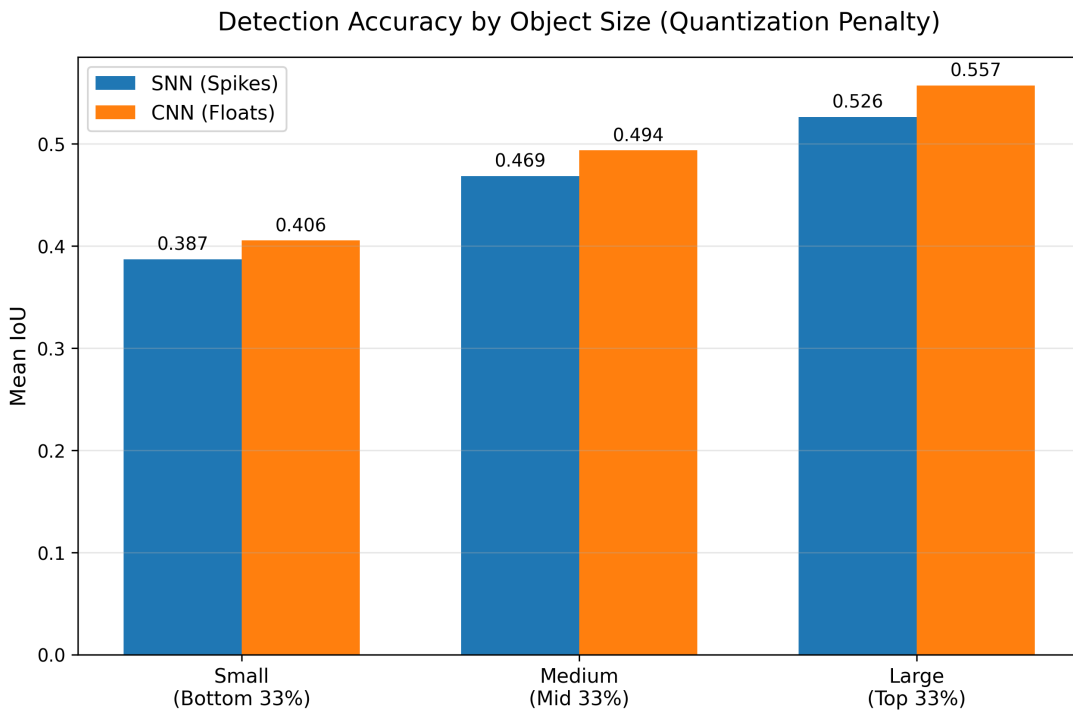
Figure 3.8: Quantization Error Analysis (Accuracy vs. Object Size) of SNN (Blue) and CNN (Orange).
