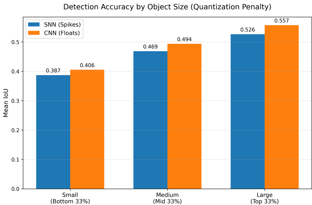
Figure 1.6: Quantization Error Analysis (Accuracy vs. Object Size) of SNN (Blue) and CNN (Orange).
