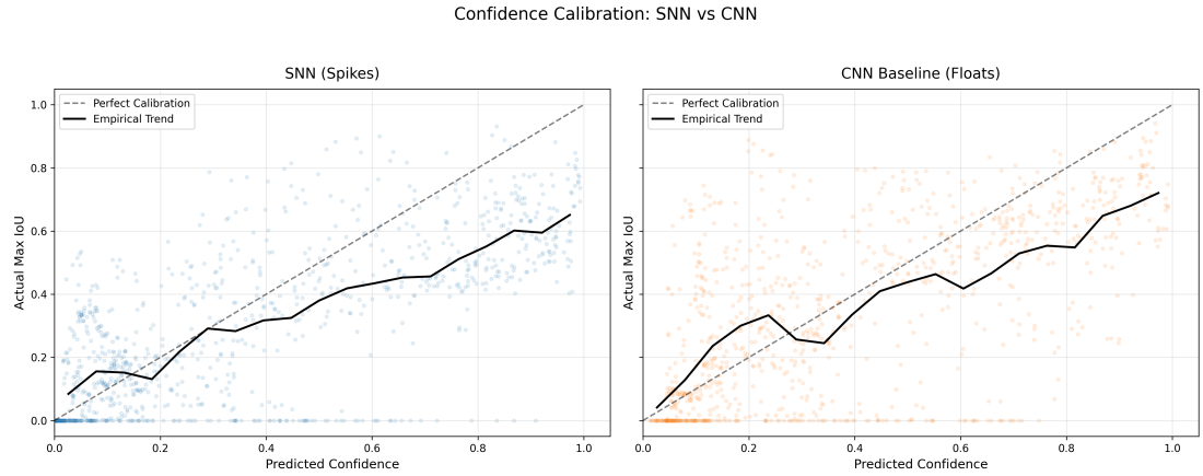
Figure 1.7: Reliability diagrams for the SNN (left) and CNN (right). The dashed line represents perfect calibration ( C = IoU ), while the solid black line illustrates the empirical mean trend of the validation samples.
