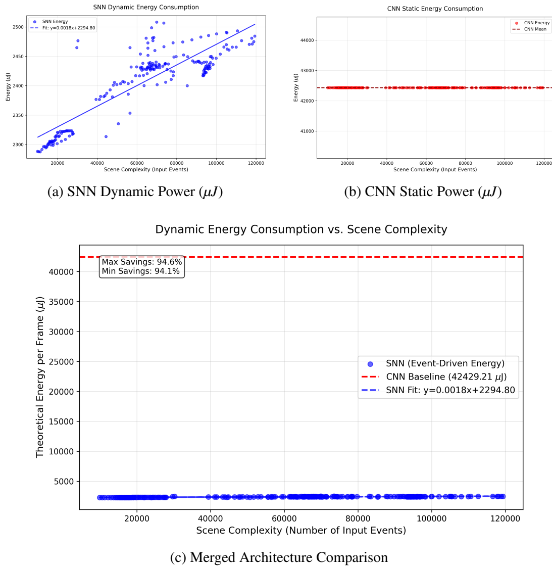
Figure 1.5: Comparison of dynamic power consumption ( \mu J ) between the SNN and CNN architectures relative to the raw event count of the input scene. The isolated SNN graph (a) demonstrates strong linear scaling ( R^2 = 0.7514 ), validating its event-driven efficiency, whereas the CNN (b) consumes a massive static overhead.
