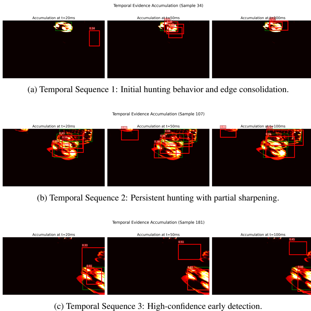
Figure 1.9: Evolution of SNN bounding box predictions over T = 10 timesteps, with annotated confidence scores. Each row demonstrates the progression from sparse initial evidence to a stable, high-confidence detection.
