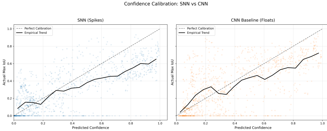
Figure 1.8: Reliability diagrams for the SNN (left) and CNN (right). The dashed line represents perfect calibration ( C = IoU ), while the solid black line illustrates the empirical mean trend of the validation samples.
