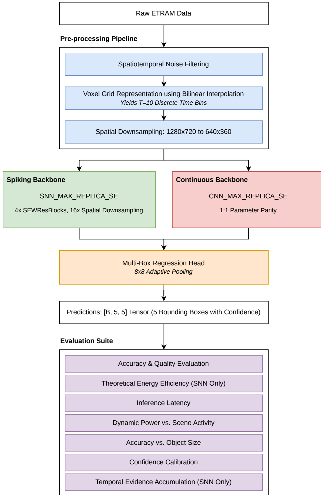
Figure 2.1: The high-level system architecture pipeline, illustrating the flow from raw ETRaM high-definition event data, through the fixed REPLICA preprocessing stages, into the interchangeable neural backbone (SNN or CNN), and concluding with the multi-box regression head and the comprehensive evaluation suite.
