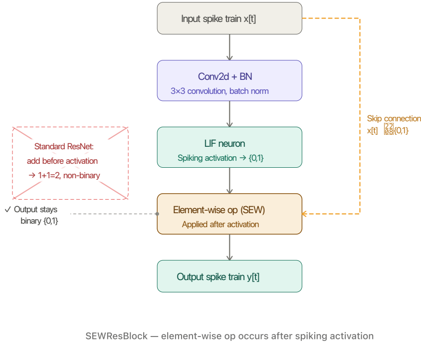
Figure 2.3: The SEW residual block (SEWResBlock) as proposed by [9].
