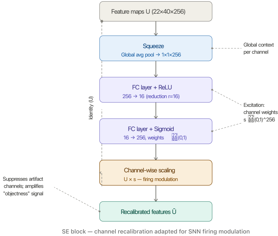
Figure 2.4: The Squeeze-and-Excitation (SE) block [16] as applied in Stage 3 of the SNN_MAX_REPLICA_SE backbone ( 22 \times 40 \times 256 ).
