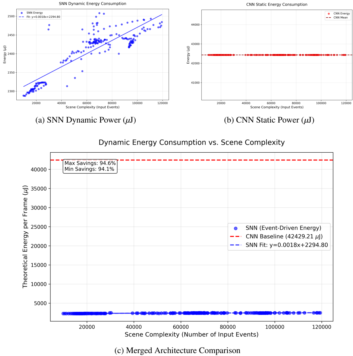
Figure 4.3: Comparison of dynamic power consumption ( \mu\text{J} ) between the SNN and CNN architectures relative to the raw event count of the input scene. The isolated SNN graph (a) demonstrates strong linear scaling ( R^2 = 0.7514 ), validating its event-driven efficiency, whereas the CNN (b) consumes a massive static overhead.
