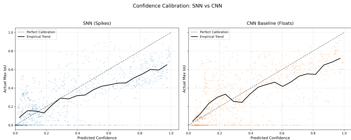
Figure 4.5: Reliability diagrams for the SNN (left) and CNN (right). The dashed line represents perfect calibration ( C = \text{IoU} ), while the solid black line illustrates the empirical mean trend of the validation samples.
