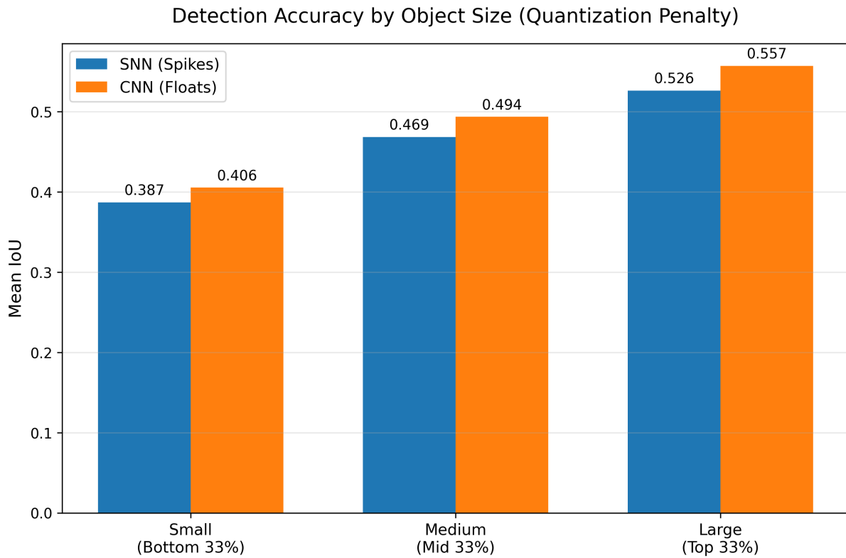
Figure 3.10: Quantisation Error Analysis (Accuracy vs. Object Size) of SNN (Blue) and CNN (Orange).
