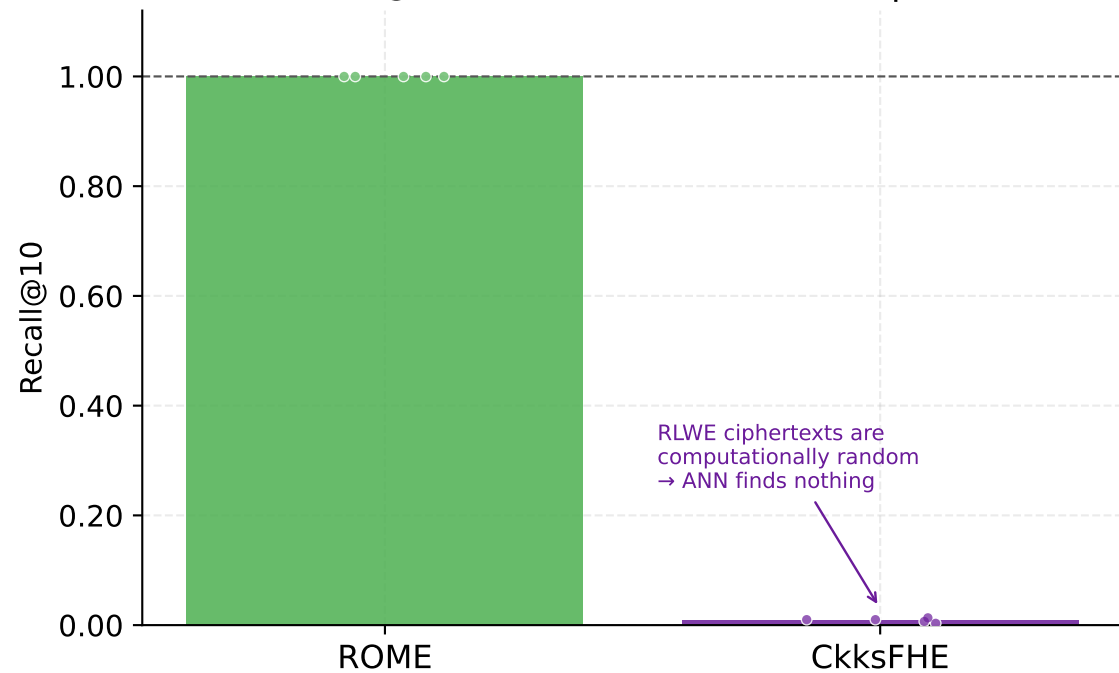
(a) Recall@10: ANN search on RLWE ciphertexts
