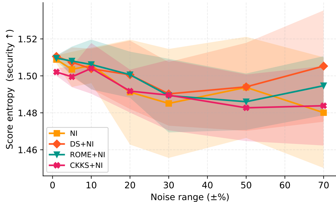
(a) Encryption Strength vs. Noise Level
