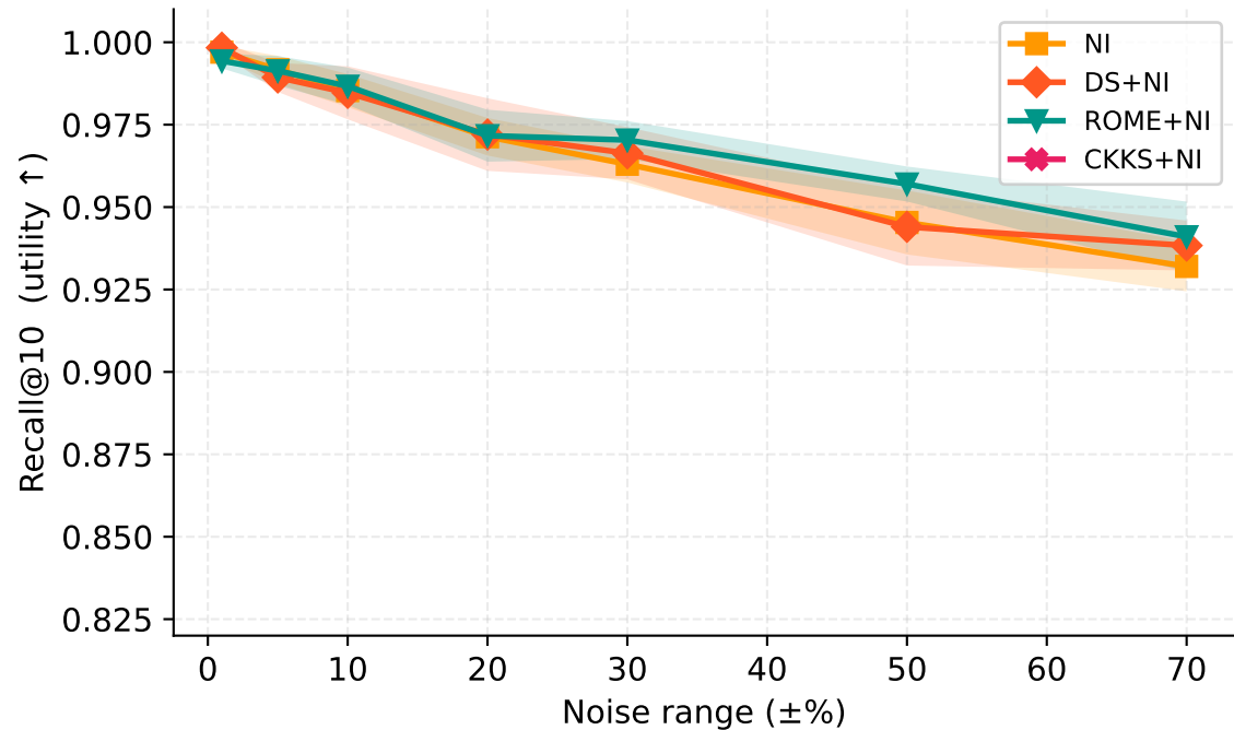
(b) Rank Preservation vs. Noise Level
