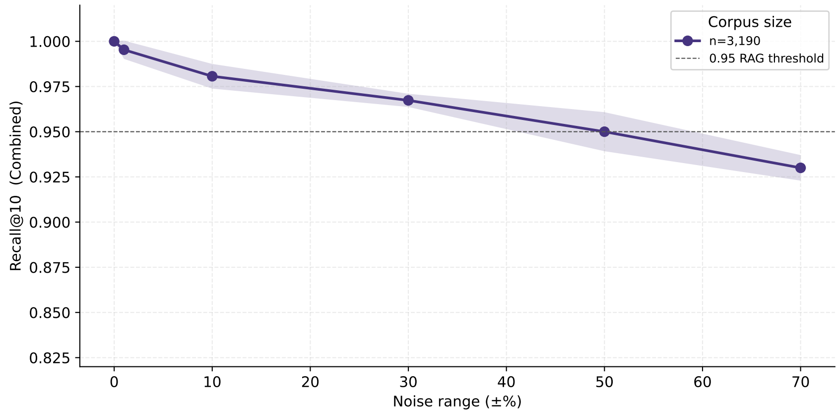
Exp I: Corpus Size \times Noise — Natural Questions (NQ) (shaded = \pm 1\sigma across trials)
