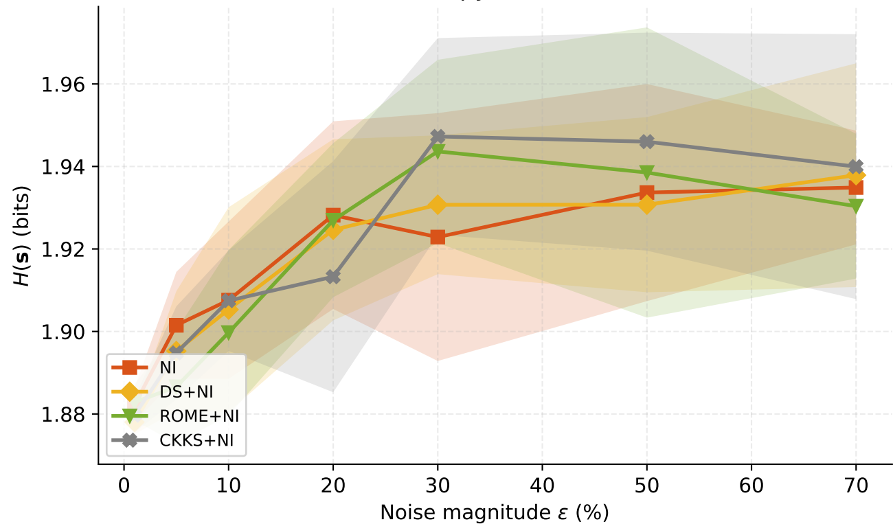
Score entropy vs. noise level
