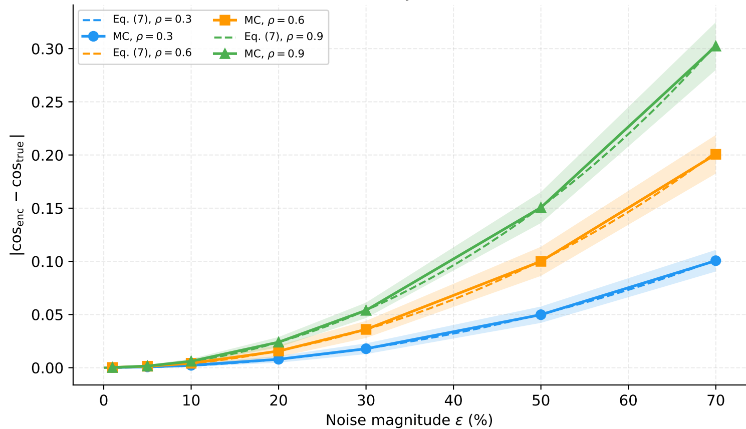
Cosine similarity distortion vs. \varepsilon
