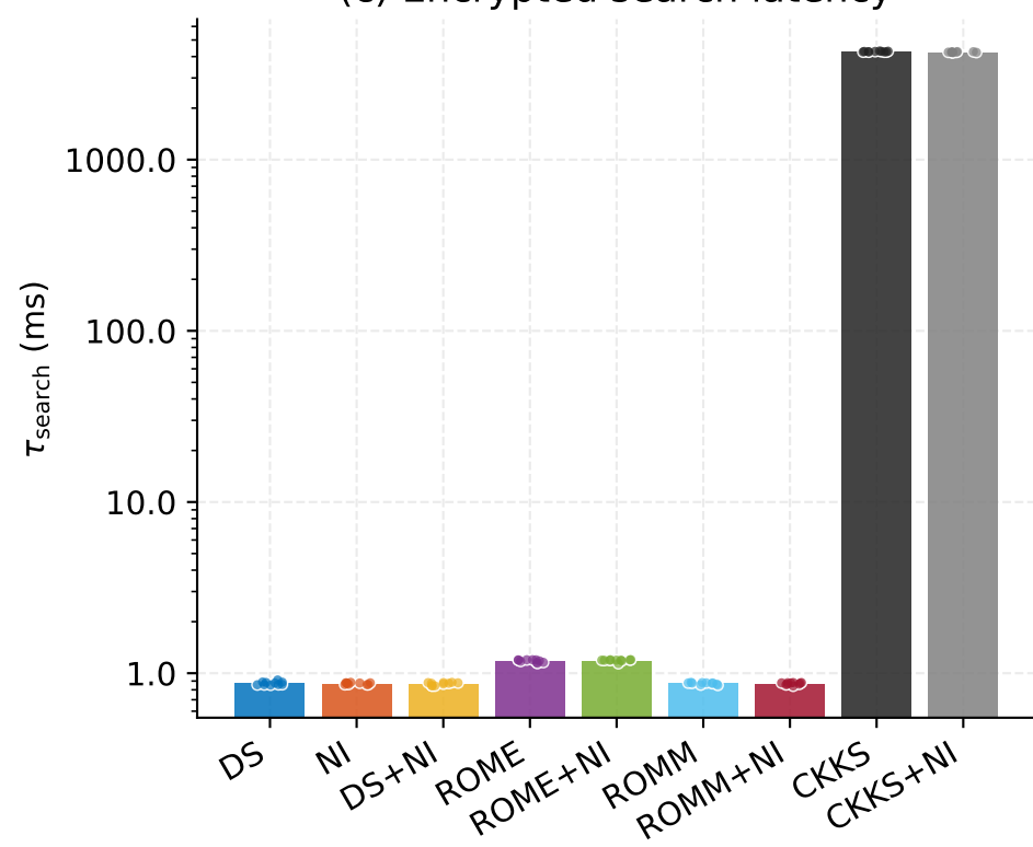
(c) Encrypted search latency
