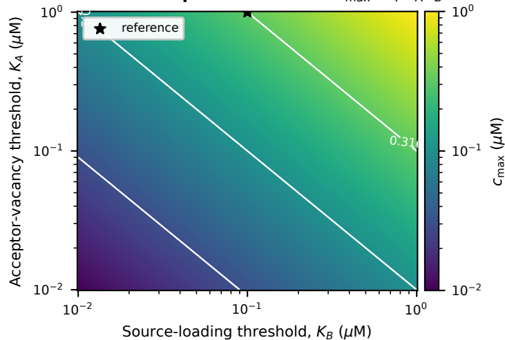
B. Window position follows c_{\text{max}} = \sqrt{K_A K_B}
