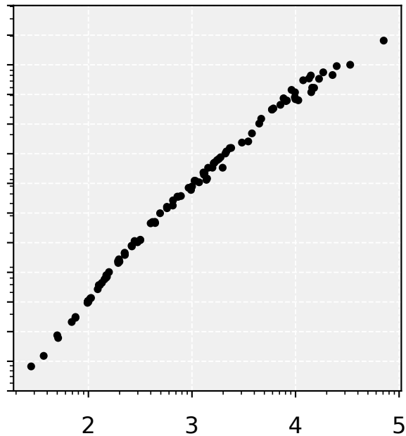
Soft VRSPD
