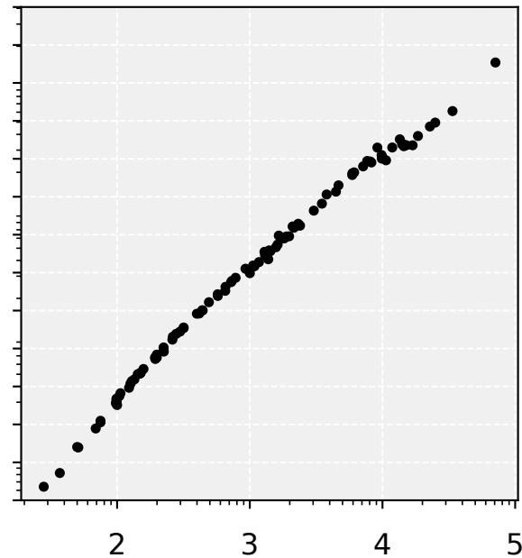
Soft VRSPDTW
