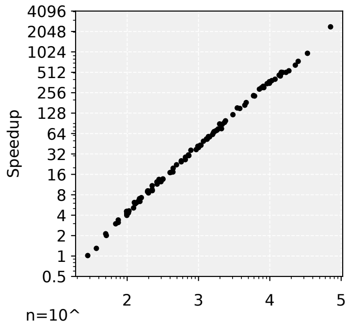
Soft VRPTW
