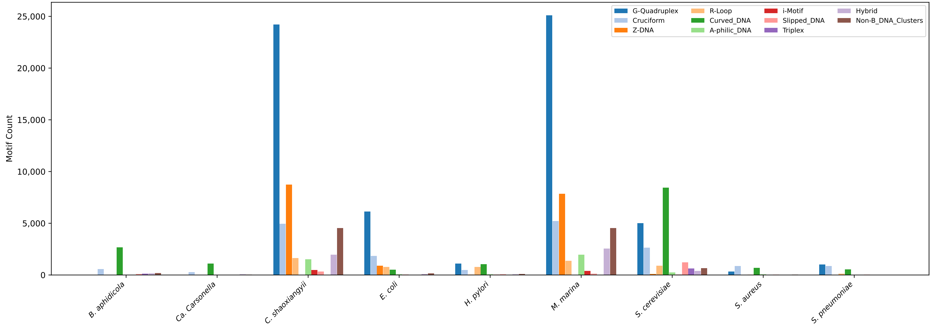
Figure 2 Non-B DNA Class Distribution Across Nine Genomes (Raw Counts)
