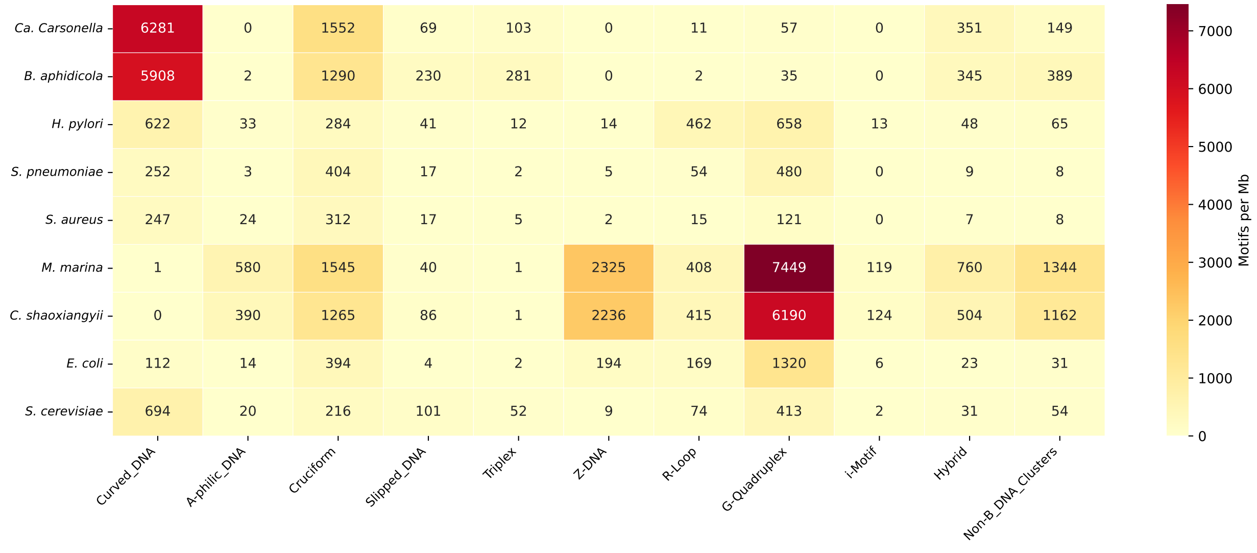
Figure 3 Non-B DNA Class Density Heatmap (motifs / Mb)
