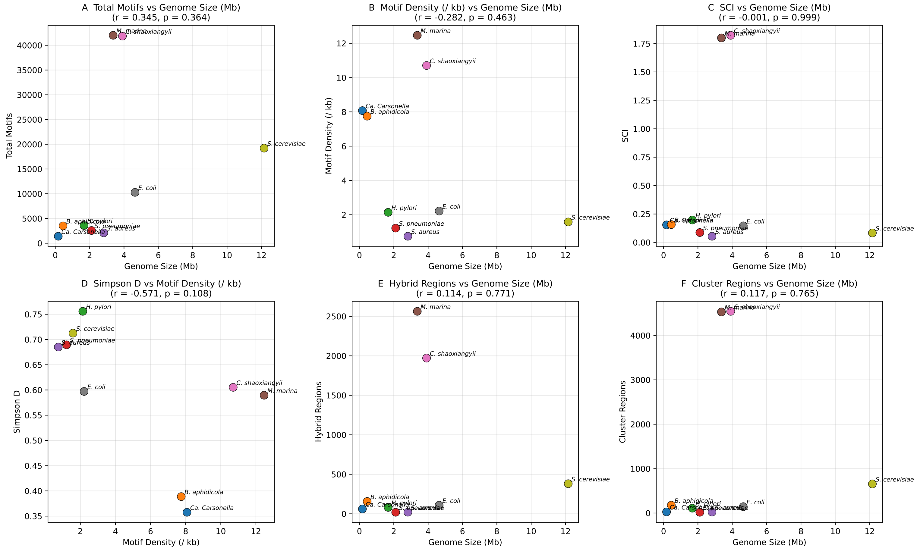
Figure 10 Genome Size vs. Non-B DNA Metrics
