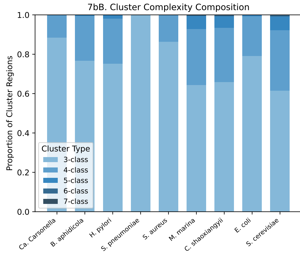
Figure 7b. Cluster Region Deep Analysis
