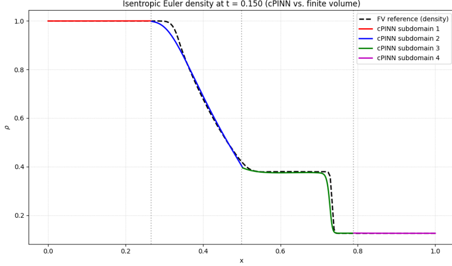
Figure 2. Density predicted by the extremum-regularized cPINN at t = 0.150 , compared with the finite-volume reference solution. The regularized model captures the principal wave structure, but its relative L^2 density error is larger than that of the baseline cPINN in the reported run.
