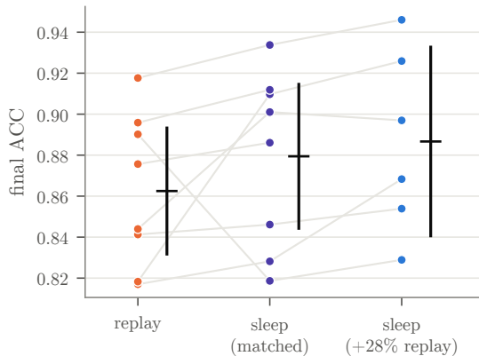
SNN+Transformer, fetch3: accuracy
