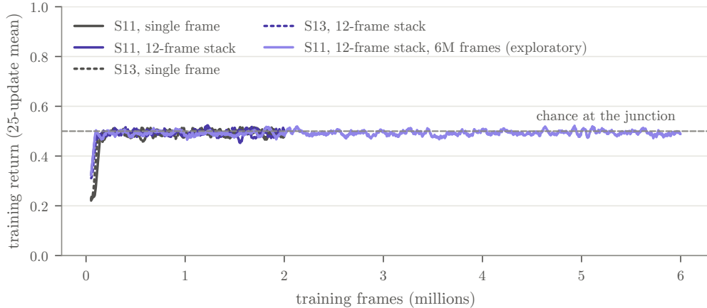
Figure 6: Memory-benchmark probes (sizing runs whose decision rule was prospectively specified; CNN encoder, one seed each, learning rate 0.0003). Training return (moving mean over 25 updates) on MiniGrid-MemoryS11 and S13 with a single frame (grey) or a stack of the last 12 frames (violet); light violet: an exploratory 6M-frame run of the stacked CNN on S11. A return of 0.5 is chance at the junction. No run learns to use the cue, so neither map tests working memory.
