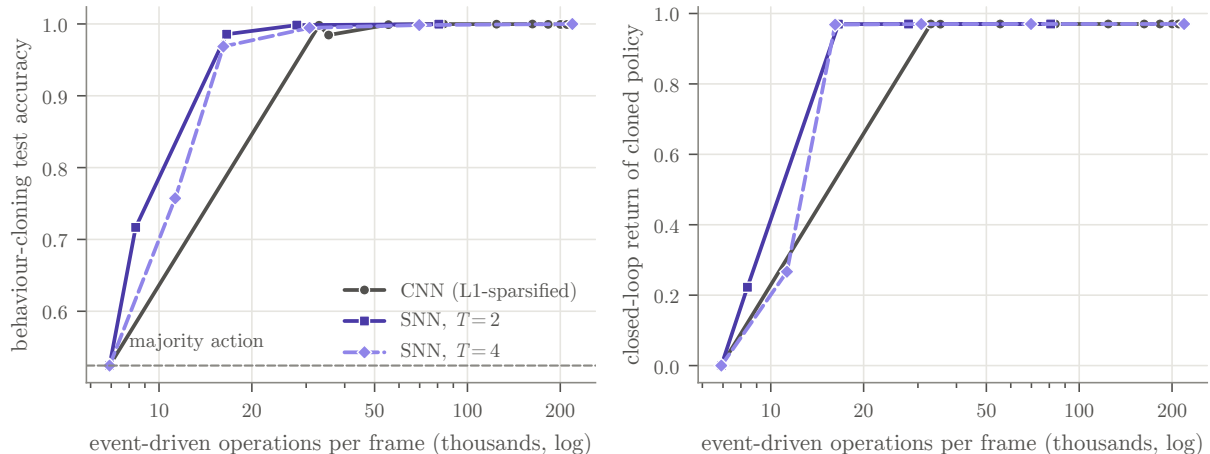
Figure 1: Accuracy against operation count for the spiking and the conventional encoder (descriptive). Each encoder, with an identical linear readout, is trained by behaviour cloning of a trained DoorKey-6x6 PPO teacher with an activity penalty; each point is one penalty value (mean of 2 seeds, the same seeds at every point). The x -axis counts event-driven operations per frame (synaptic operations for the SNN, non-zero multiply-accumulates for the L1-sparsified CNN; log scale). Left: held-out action accuracy (dashed: majority-action rate). Right: closed-loop return of the cloned policy. The SNN keeps working below the lowest operation count at which the CNN still works.
