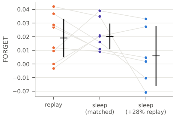
forgetting (lower is better)
