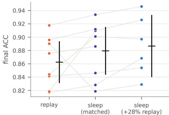
hybrid, fetch3: accuracy
